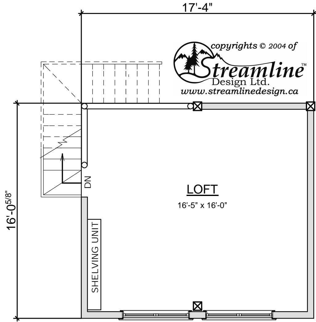
LOFT FLOOR PLAN AREA: 278 SQ. FT.
